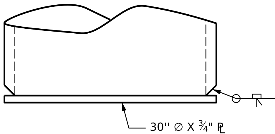
PIPE PILE PLATE DETAIL ( IF APPLICABLE )
