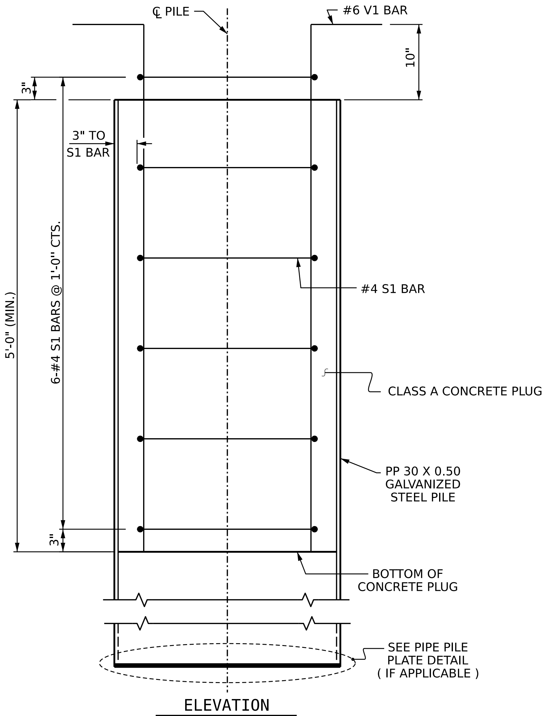
PP 30 X 0.50 GALVANIZED STEEL PILE ( OPEN OR CLOSED END )
